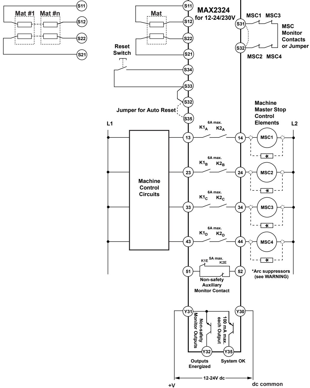
Figure 4. Hookup to a Four-Wire Safety Mat
