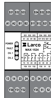
Figure 1. Indicator and Terminal Locations
